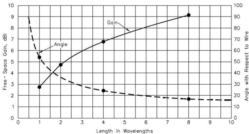
Theoretical gain of a long-wire antenna, in dBi, as a function of wire length. The angle, with respect to the wire, at which the radiation intensity is maximum also is shown.
